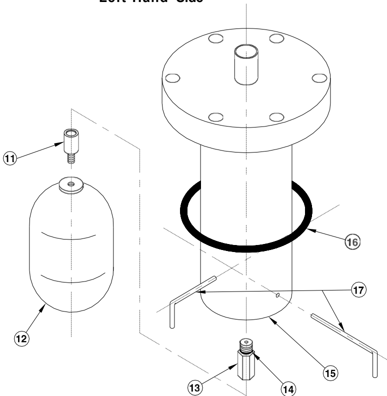
Purser Vessel Cover and Float Ball Assemblies
