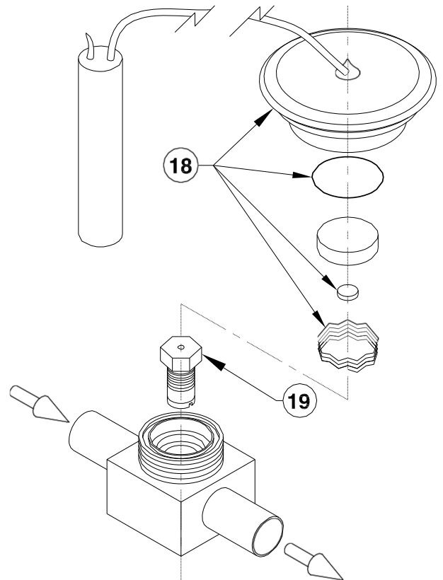
Combination Temperature/Check Valve (9)
