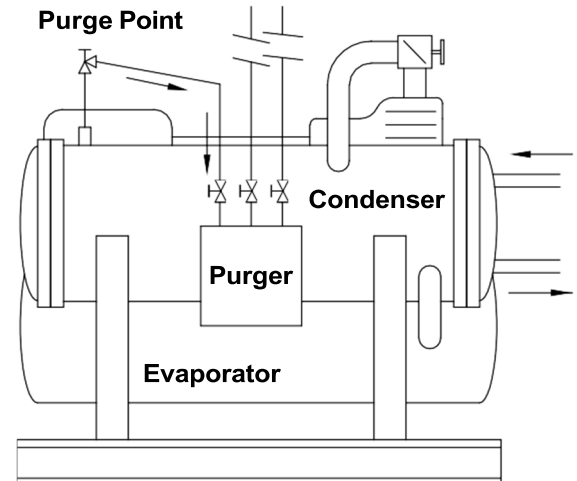
Skidded Refrigeration Package
