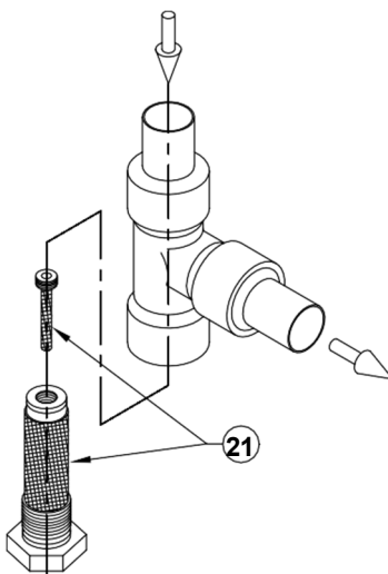
Strainer/Orifice (5a, 5b)
