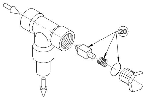
225 psid Check Valve
