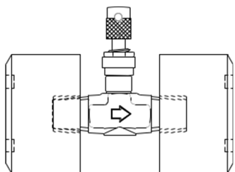
NEAPF Liquid Feed Valve (1b)
